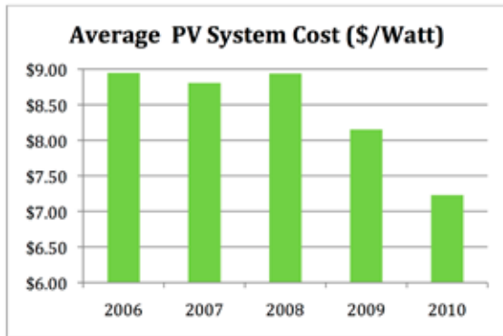
Figure 2 — Average PV system prices by year in the Oregon Residential Energy Tax Credit Program
